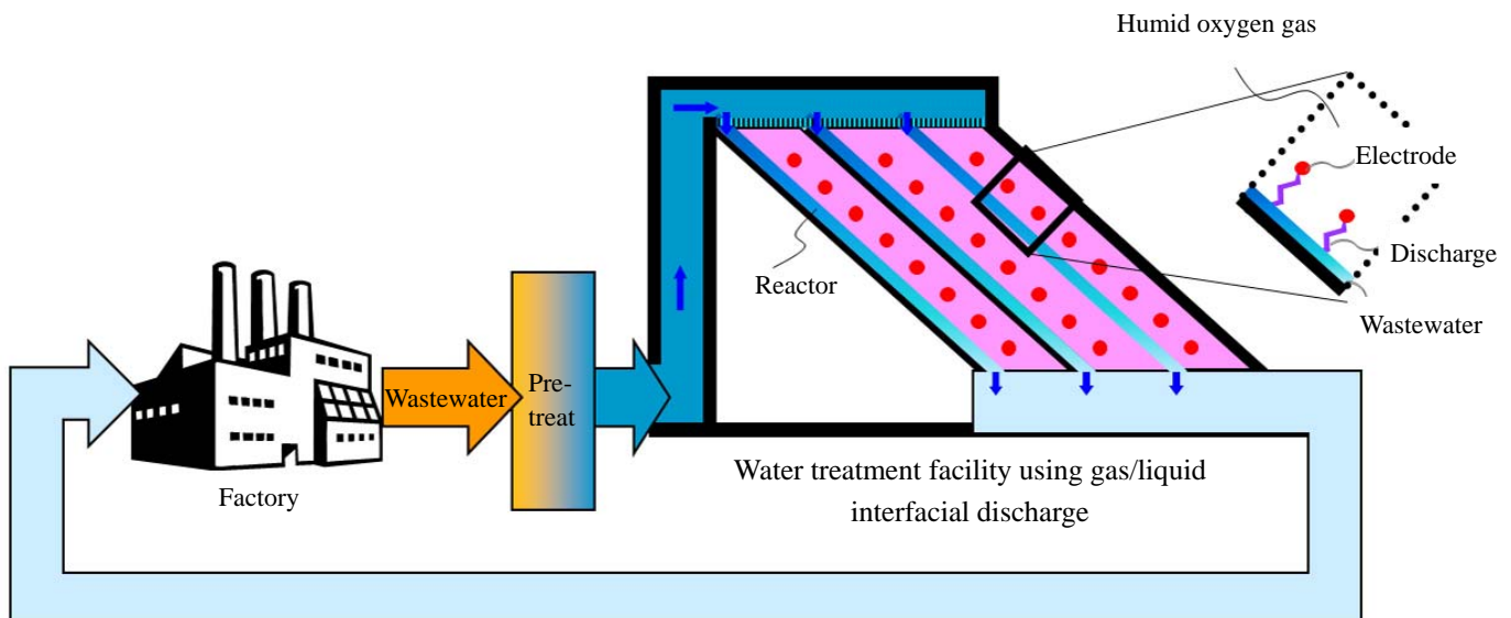
System diagram of industrial wastewater reuse using gas/liquid interfacial discharge technology
